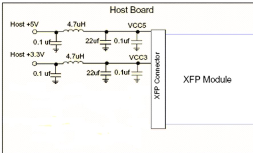
Figure 5 Example of Host Board Supply Filtering Network
