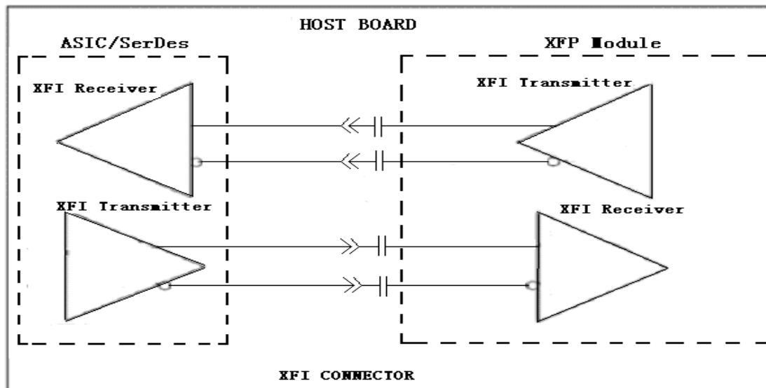
Figure 1 High Speed Electrical Interface
