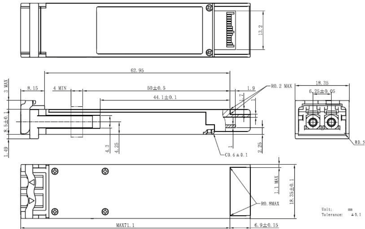
Figure 6 Package Outline
