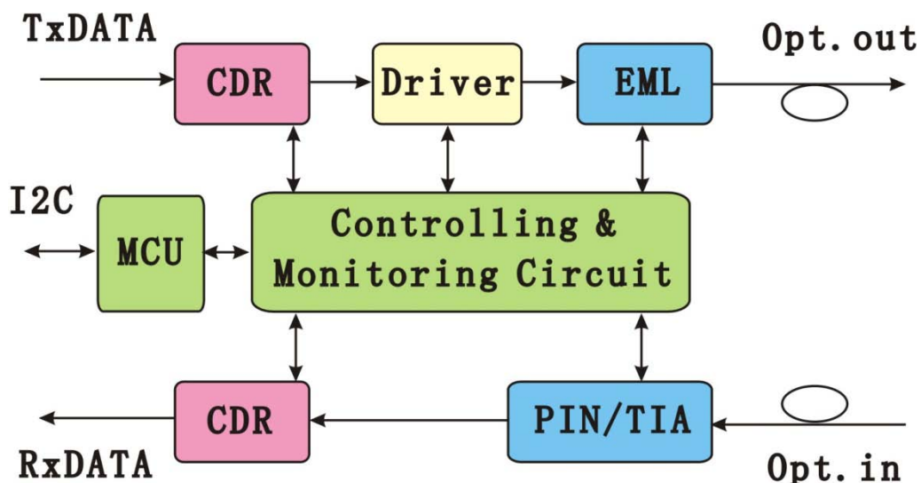
Figure 3 Block Diagram for RTX226-440
