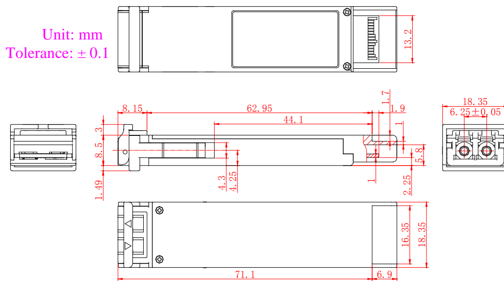
Figure 6 Package Outline
