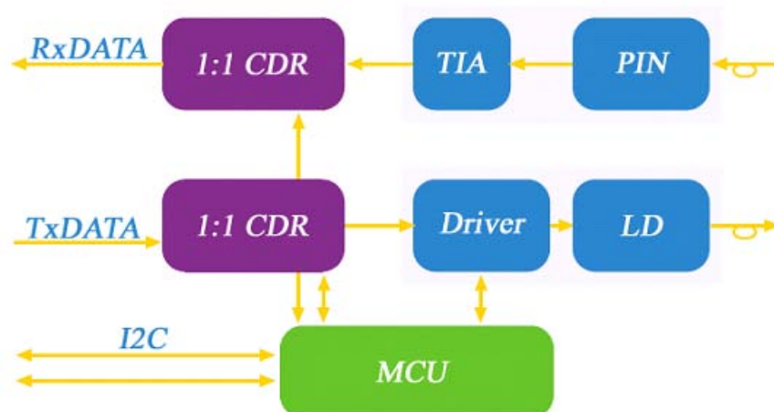
Figure 3 Block Diagram
