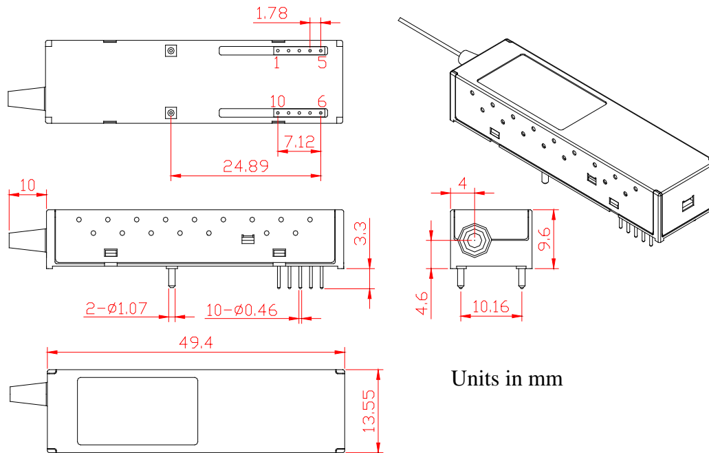
Figure5 Package outline
