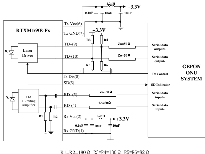
Figure4 Typical application circuit
